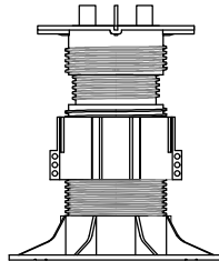
LC + C4 6 1/4" - 8 3/4" VERTICAL RANGE (159mm - 222mm)
