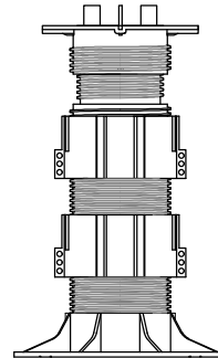
LC + C4 + C4 8 3/4" - 12" VERTICAL RANGE (222mm - 305mm)
